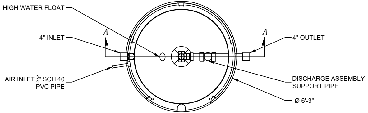
TOP VIEW DETAIL (COVER REMOVED)
