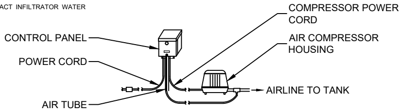
AIR COMPRESSOR HOUSING & CONTROL PANEL ASSEMBLY SCALE 1:40
