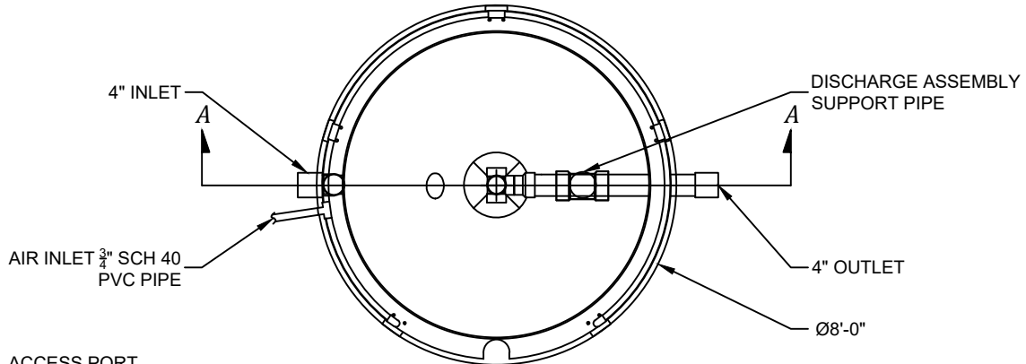
TOP VIEW DETAIL (COVER REMOVED)
