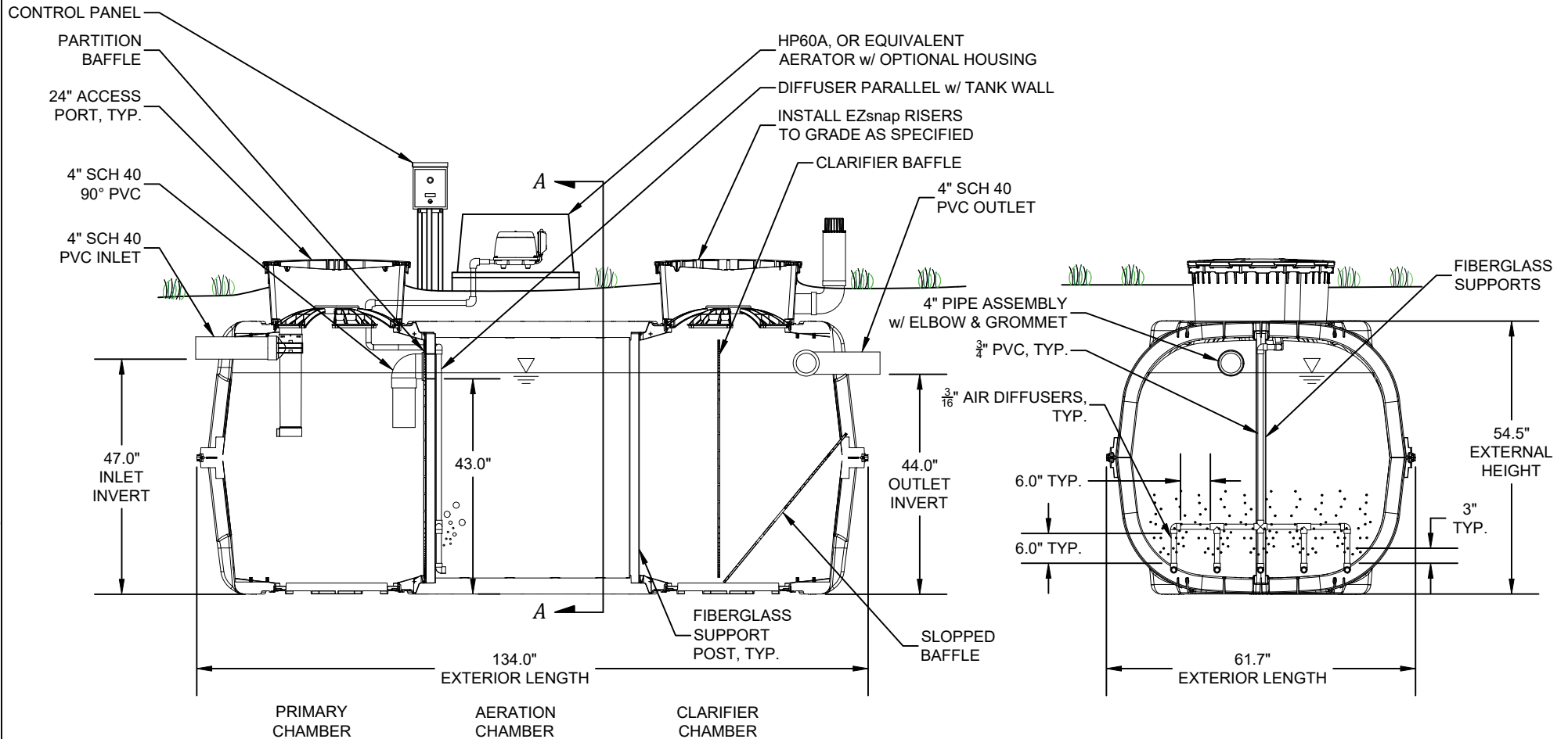
SIDE VIEW SECTION A-A
