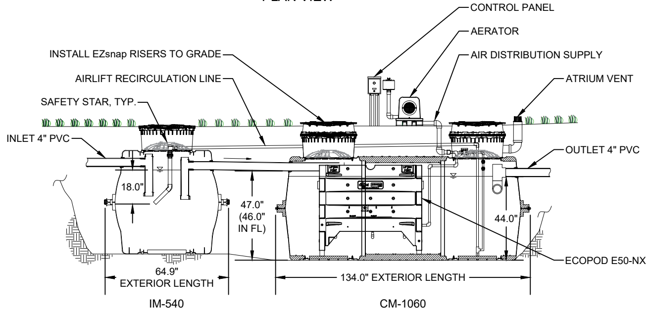
ELEVATION VIEW
